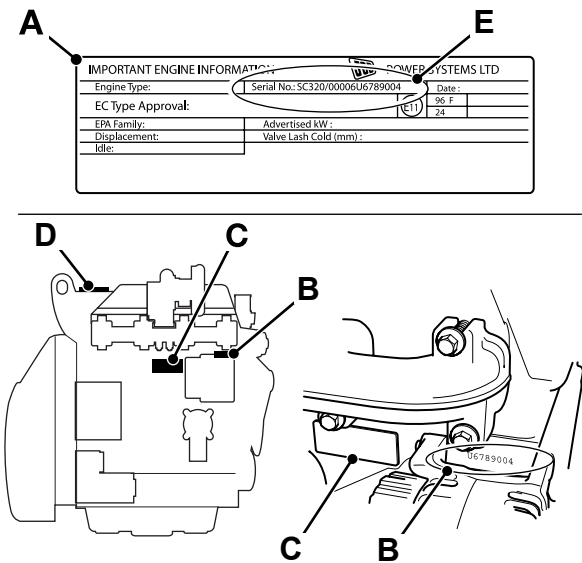
Fig 3. Engine
