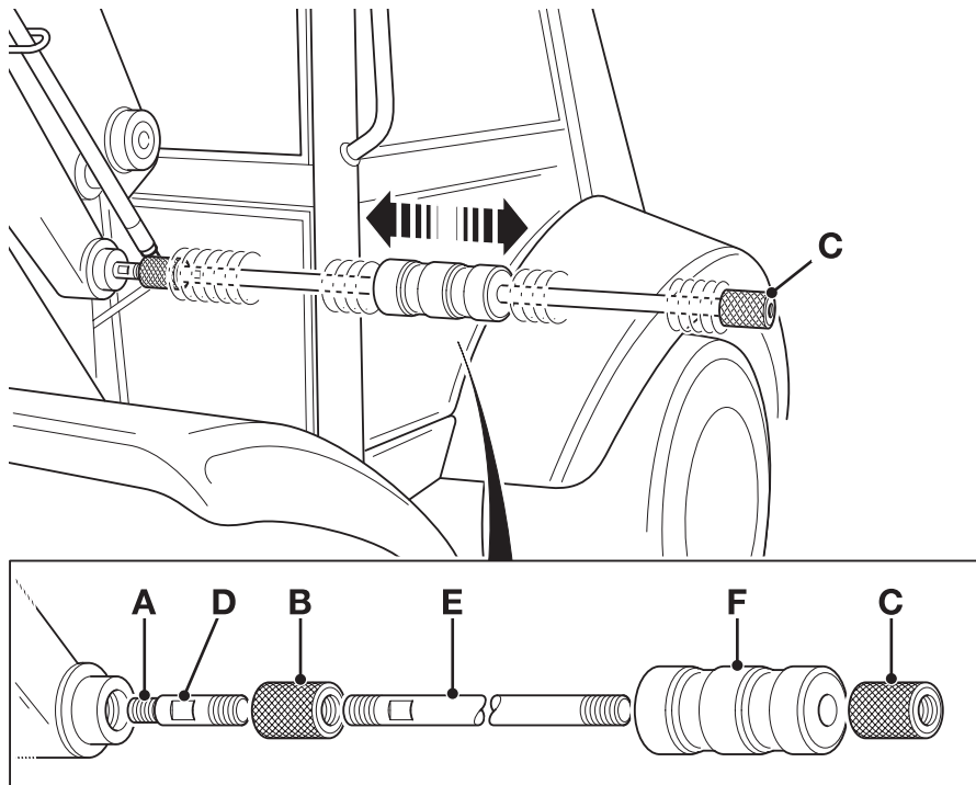
Fig 76. Typical M/c. Installation
