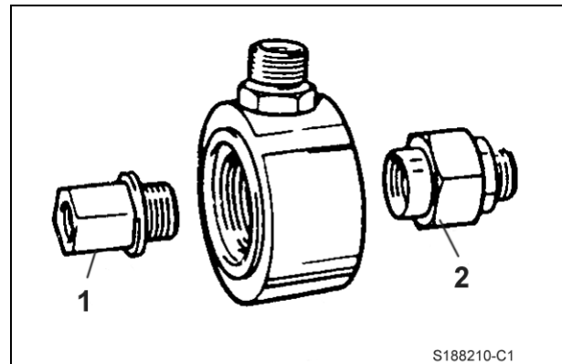
Fig 44. 892/00301 Flow Test Adaptor
