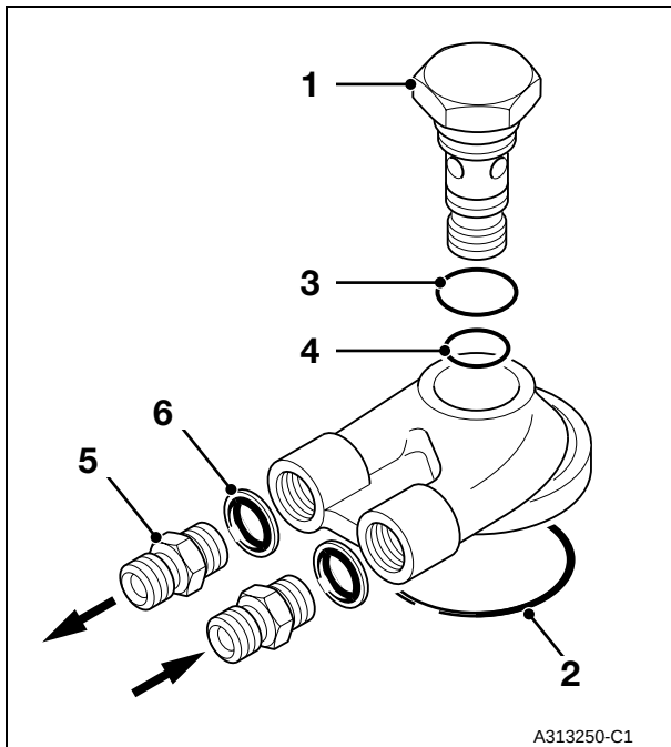
Fig 43. 460/15708 Flow Test Adaptor
