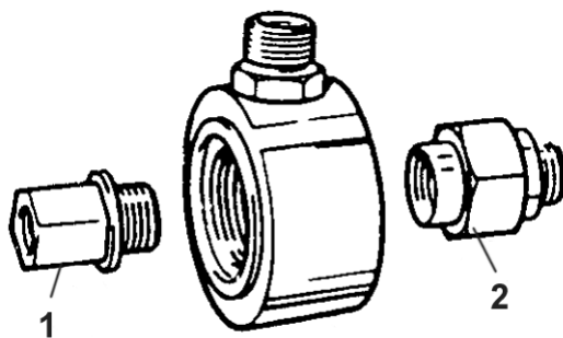
Fig 57. 892/00301 Flow Test Adaptor
