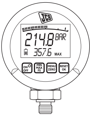
Fig 42. 892/01268 Digital Pressure Gauge 0-400 bar
