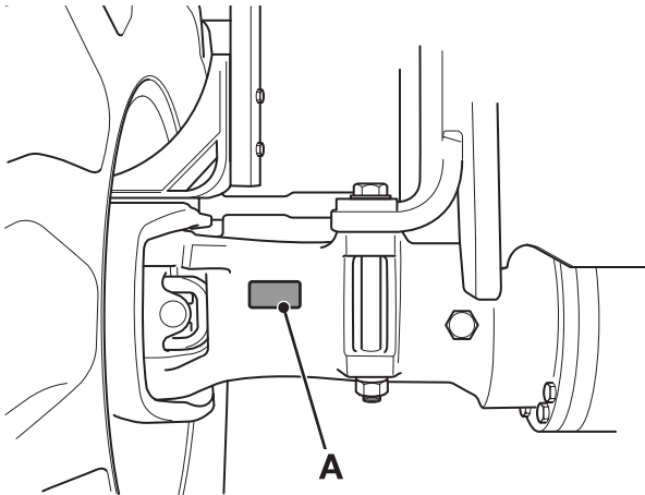
Fig 4. Front Axle
